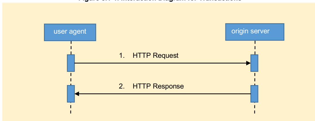
825 Figure 8.1-1. Interaction Diagram for Transactions
